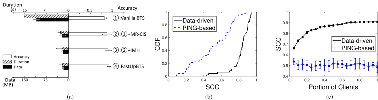
Fig. 9. (a) Impact of individual modules of FastUpBTS on top of the edge-to-cloud testbed. (b) Distributions of SCC_{gp} (PING-based) and SCC_{gd} (Data-driven) when P=20\% ; (c) P (portion of clients) vs. SCC_{gp} and SCC_{gd} .
