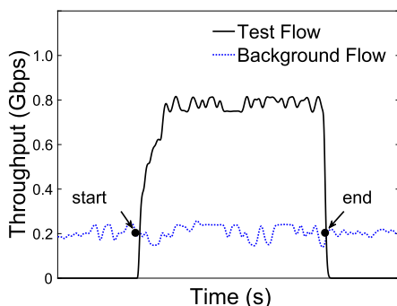
Fig. 10. Evaluating the probing intrusiveness of FastUpBTS.
